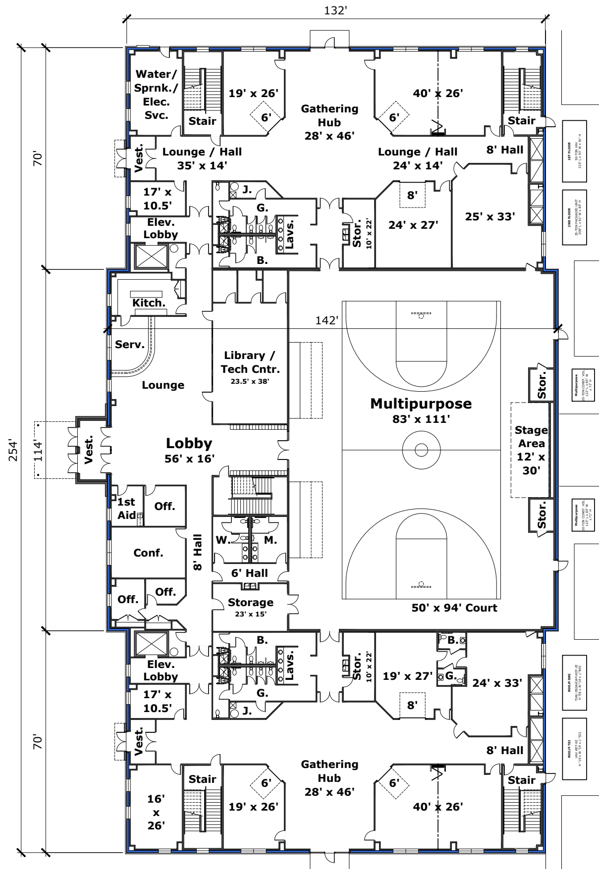
1st Floor 34,063 sf
