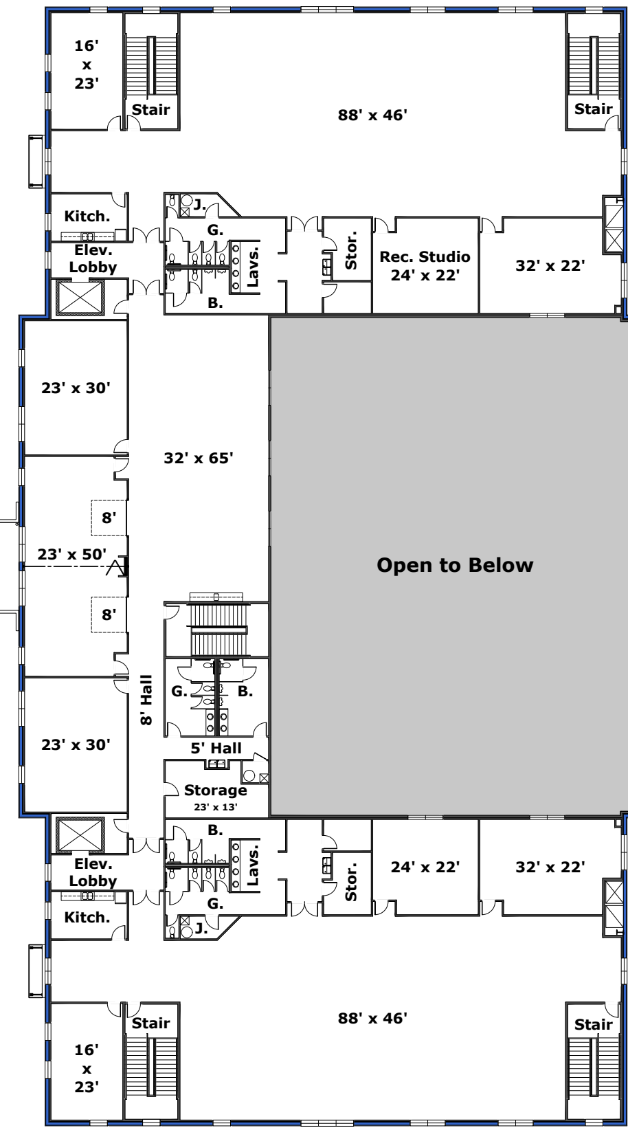
2nd Floor 22,768 sf
